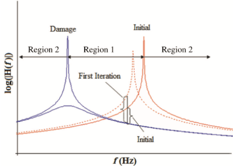
Figure 4. TF of an intact and damaged structures.
