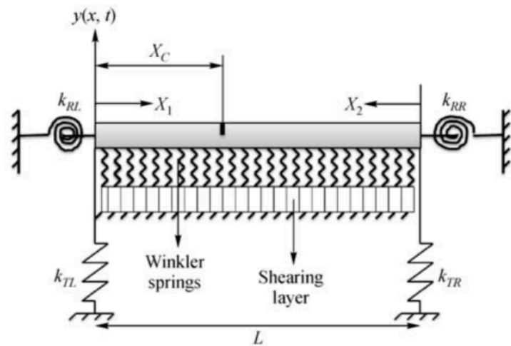
Fig. 1 Cracked beam with elastically restrained ends resting on two-parameter elastic foundation
