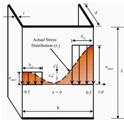
Figure 1. Longitudinal stress approximation.
