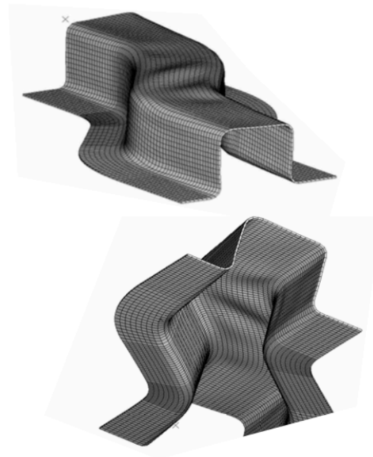
FIGURE 5. Deformed configuration, with the onset of wrinkles in the final aluminum alloy part (top and bottom views)
