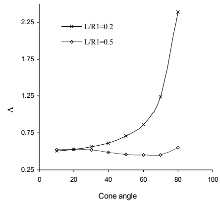
Fig. Critical load ratio for isotropic SS3 conical shell ( h/R1=0.01 ; N=15 )
