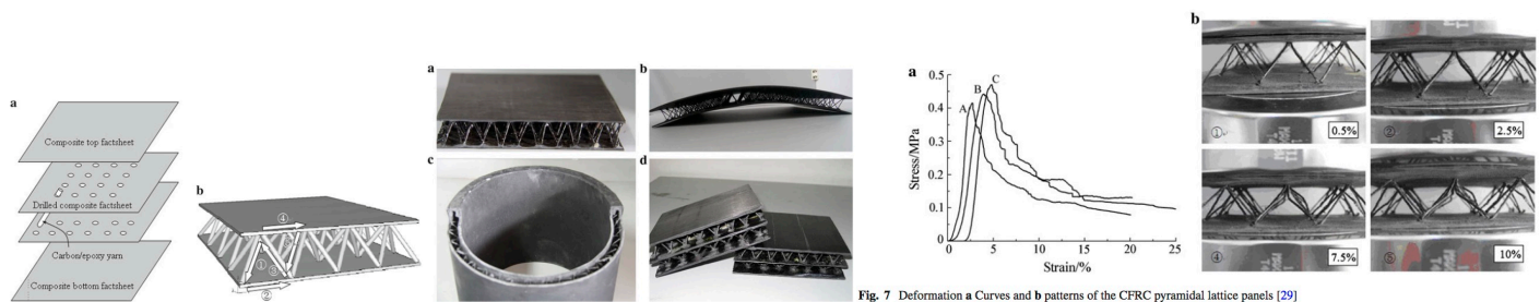
Fig. 7 Deformation a Curves and b patterns of the CFRPC pyramidal lattice panels [29]
