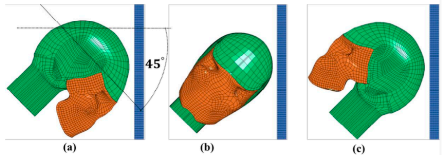
FIGURE 2: SCENARIOS FOR THE HEAD IMPACT AGAINST THE RIGID WALL; (A) FRONT IMPACT; (B) SIDE IMPACT; AND (C) BACK IMPACT
