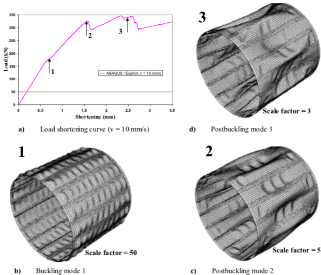
FIGURE 4. Pure axial loading
