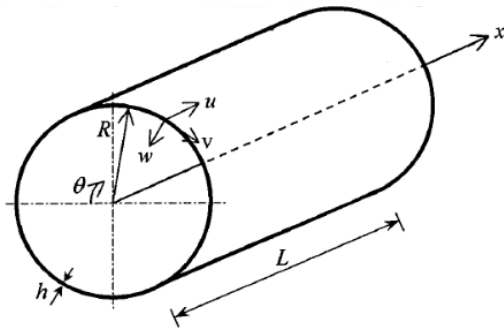
Figure 2.1 shows a circular cylindrical shell with the co-ordinate system and the displacements of the middle surface.
