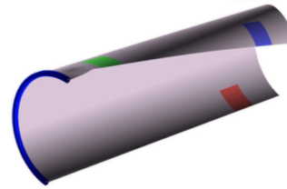
buckling of a cylindrical shell with three piezoelectric patches
