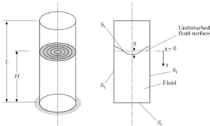
Figure 8: Sloshing model of a vertical shell
