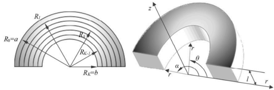
FGM cylindrical panel and coordinate system.
