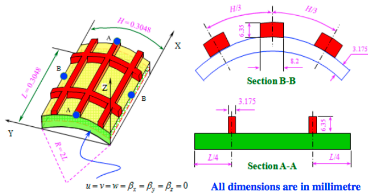
Fig. 14. A clamped-free eccentric stiffened shell.
