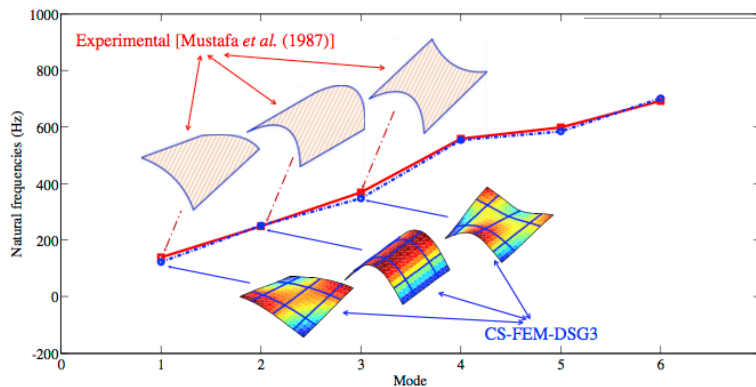
Fig. 15. Six first natural frequencies (Hz) of the orthogonally stiffened free-free cylindrical shell panel.
