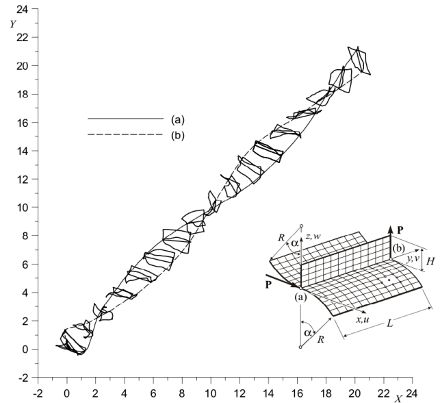
Fig. 6.13. The octant panel of the hemisphere: deformed configurations at specified time instants Fig. 6.15. Motion trajectories of the points (a) and (b) and the shape of the wavy cylindrical branched panel
