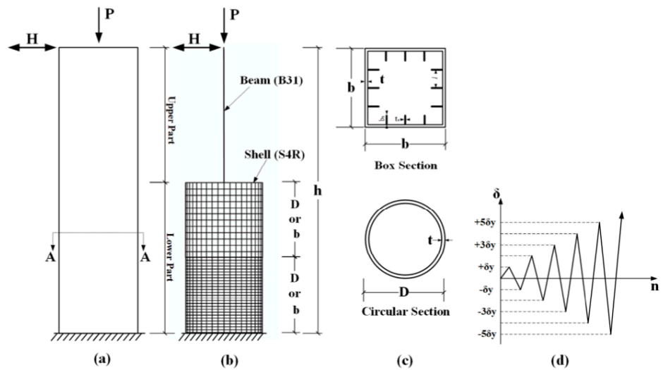
Figure 1: Analytical Model: (a) Bridge Pier; (b) FE Model; (c) Cross Sections; and (d) Loading Program
