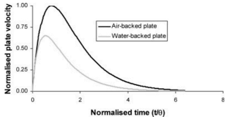
Fig. 2 Variation of normalized plate velocity as a function of normalized time for air- and water-backed plates
