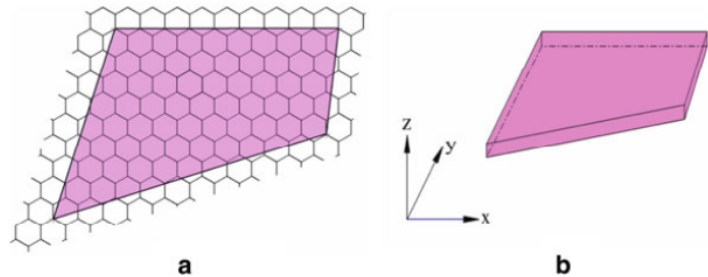
Model of quadrilateral single-layered graphene sheet. a discrete model; b continuum model
