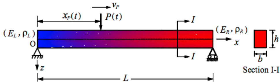
Figure 1 An axially functionally graded (AFG) simply-supported beam subjected to a concentrated moving harmonic load.
