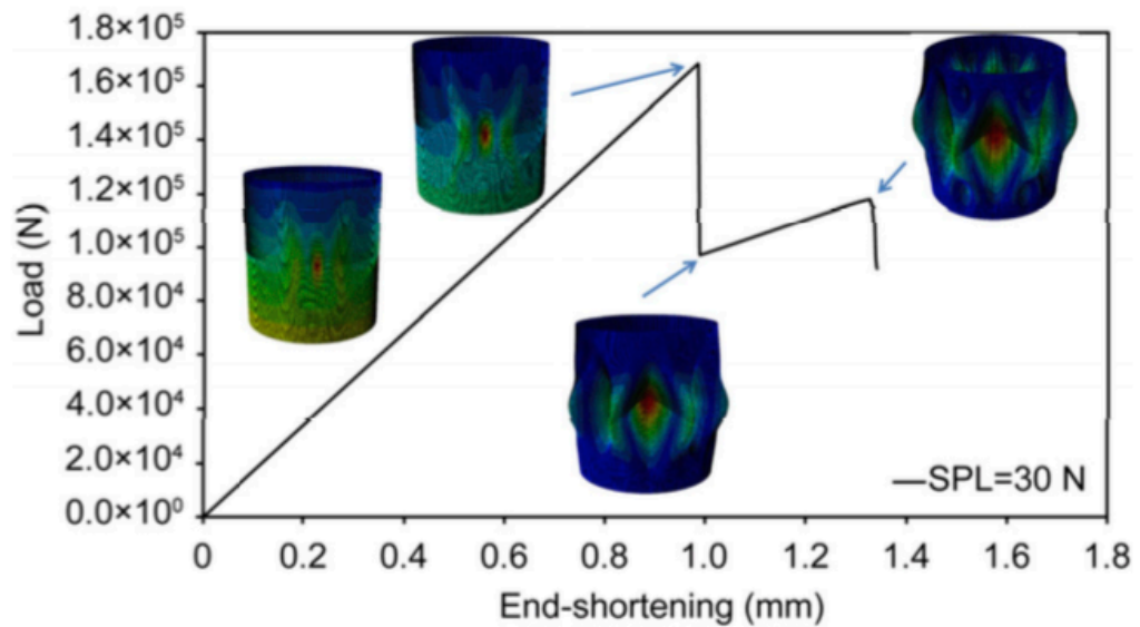
Figure 6 (Color online) Deformations of cylinder A, along the load-shortening curve.
