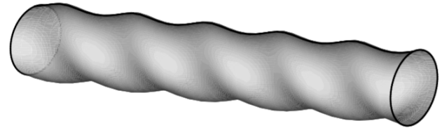
Figure 1.7: Example of Buckling Mode under Torsion
