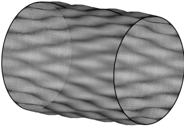
Figure 1.3: Example of Buckling Mode under Axial Compression
