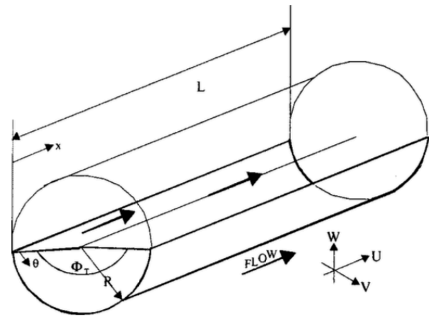
Fig. 1 Flowing fluid open cylindrical shell
