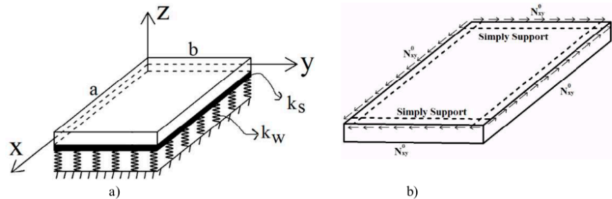
Figure 2. Geometry and boundary conditions of steel foam sandwich panels resting on Pasternak foundation
