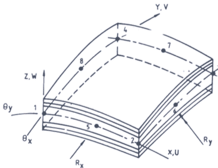
Figure 1 Geometry of a laminated curved shell.
