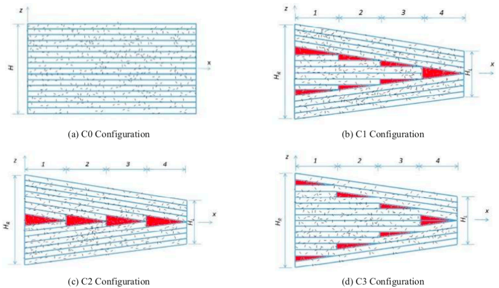
Fig. 2 Representation of various tapered configurations
