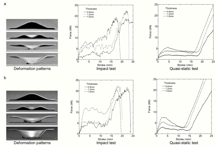
Fig. 4. Progressive deformation patterns of hemispherical top shell and force curves: (a) SS; (b) SF deformation condition.
