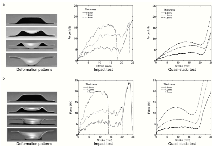
Fig. 3. Progressive deformation patterns of flat top shell and force curves in indentation, (a) FS; (b) FF deformation condition.
