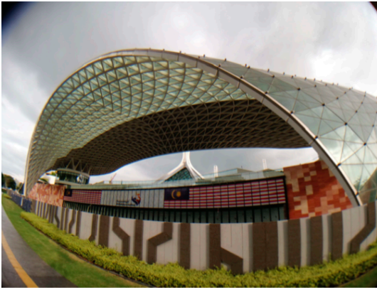
Fig.1 Latticed shell made of H-shaped steel
