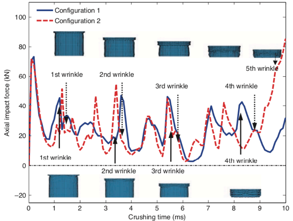
From: Shujuan Hou, Zhidan Zhang, Xujing Yang, Hanfeng Yin and Qing Li, “Crashworthiness optimization of new thin-walled cellular configurations”, Engineering Computations: International Journal for Computer-Aided Engineering and Software , Vol. 31, No. 5, pp 879-897, 2014
