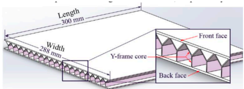
Figure 1. Schematic of the Y-frame core sandwich panel.
