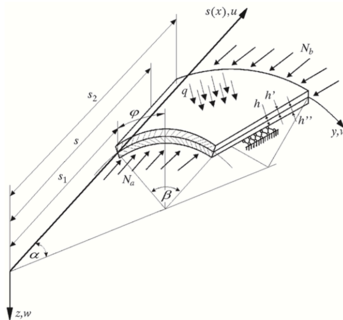
Fig. 1. Subject of consideration – bilayered open conical shell
