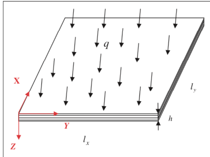
Figure 2. Laminated composite plate subjected to uniform transverse load.
