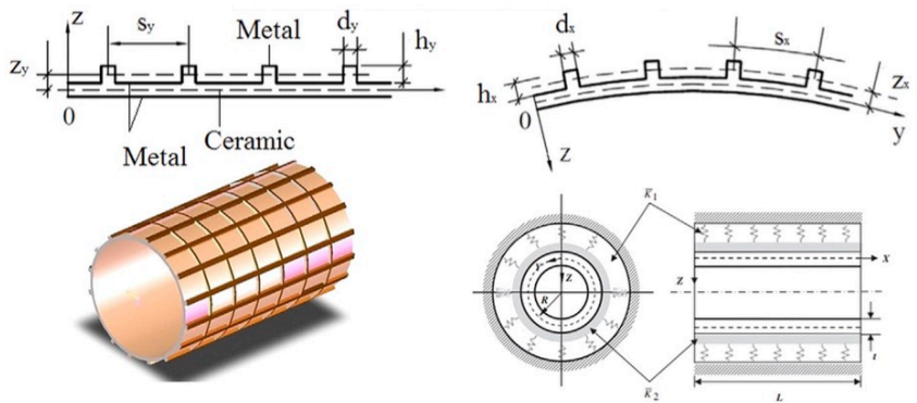
Fig. 1. Configuration of an eccentrically stiffened S-FGM circular cylindrical shell.
