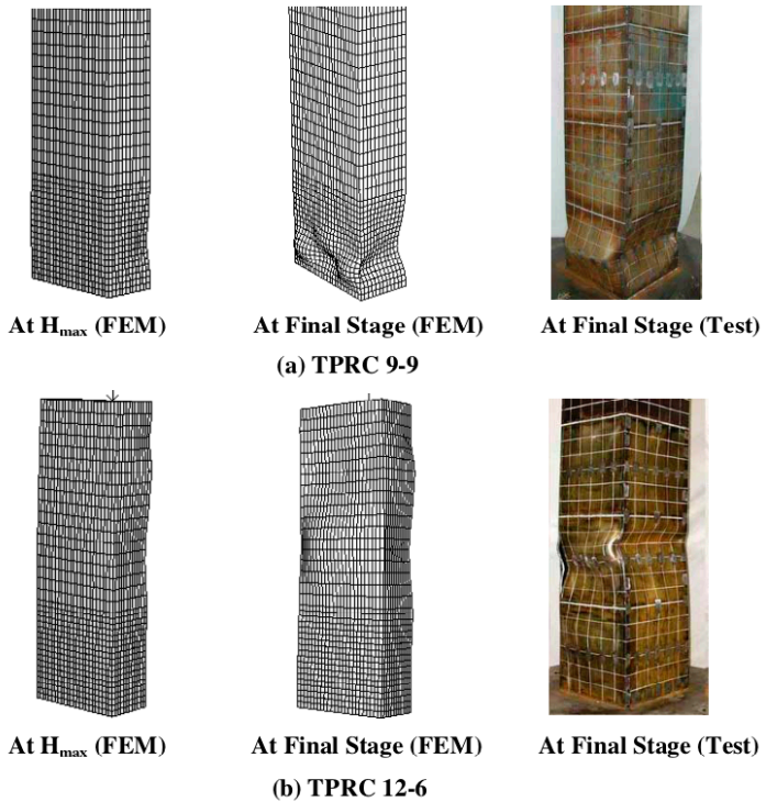
Fig. 7 Deformed Shapes of Specimens (a) TPRC 9-9; and (b) TPRC 12-6 at H_{max} and Final Stage of Test
