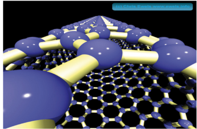
Figure 1 Nanotube [1]
