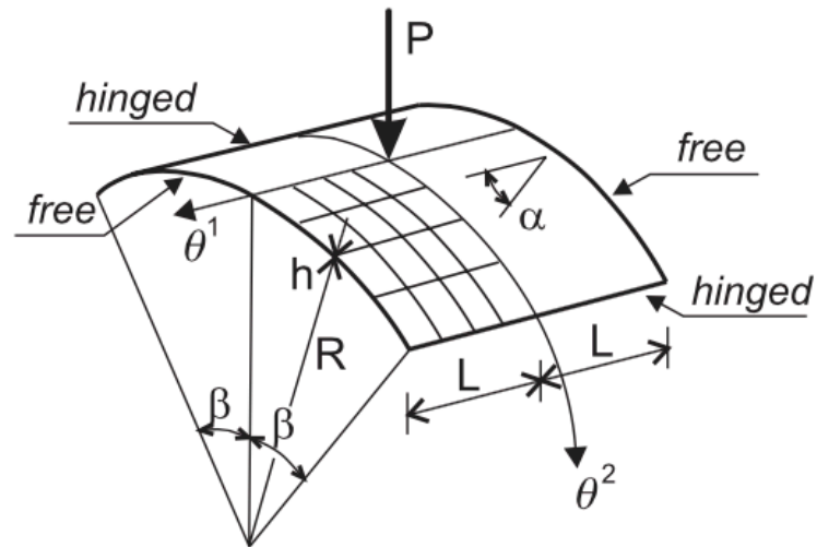
Figure 1. Hinged cylindrical panel under point load
