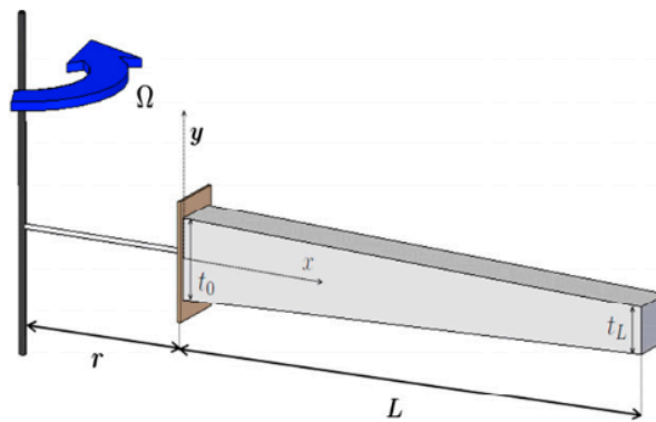
(a) Rotating nanocantilever
