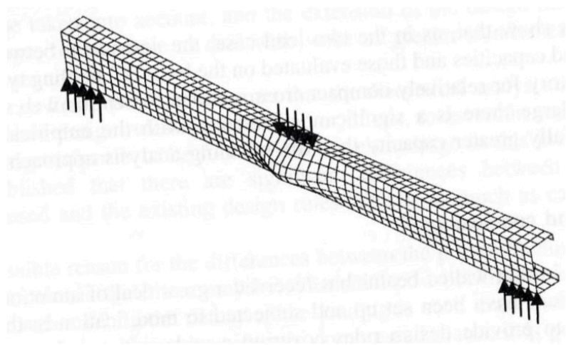
Early finite element reproduction of beam subject to web crippling
