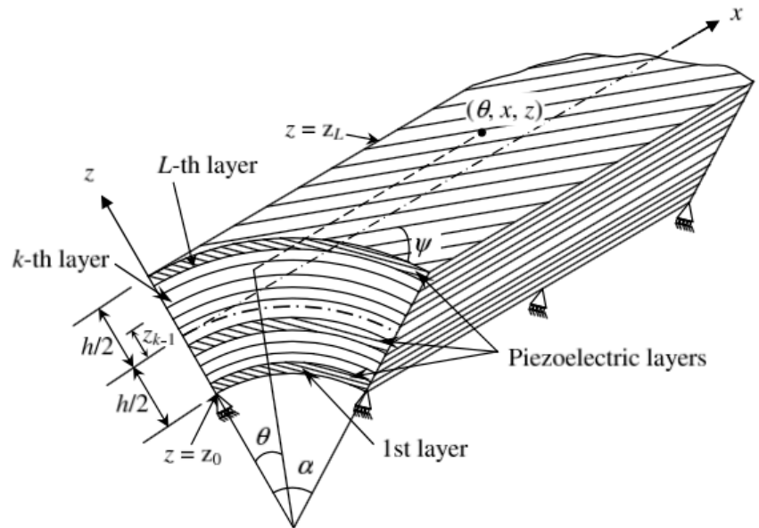
Figure 1. Geometry of a hybrid angle-ply cylindrical shell.
