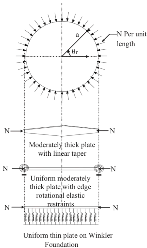
Fig. 1 Different configurations of circular plate
