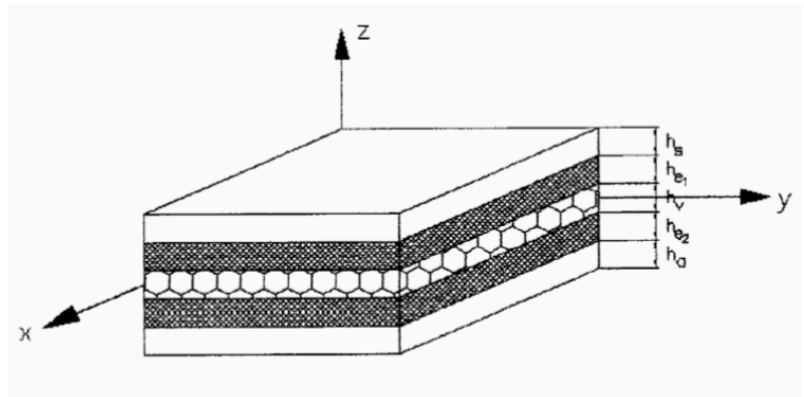
Figure 1. Sandwich plate
