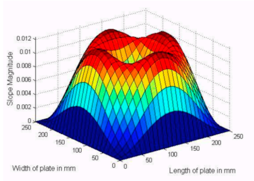
Fig.2(a) First rotational mode shape of damage plate
