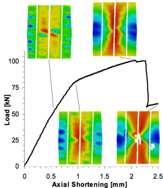
Fig. 7. Experimental load-shortening with radial displacement contours (stiffener side)
