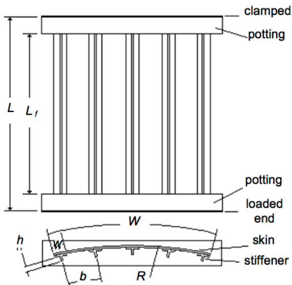
Fig. 1. Panel geometry
