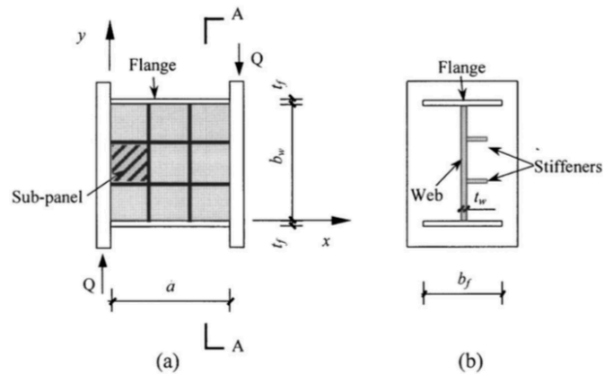
Fig. 2. Stiffened shear panel with two pairs of longitudinal and transverse stiffeners: (a) elevation and (b) view A-A
