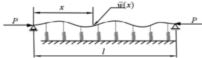
Fig. 1 A column on a nonlinear mixed quadratic-cubic elastic foundation
