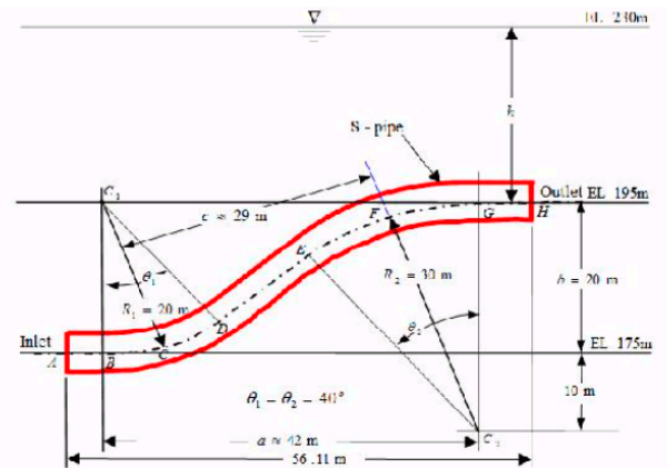
Shell S-Pipe with Inner Diameter (of the Inner Shell) d_1 = 10 m
