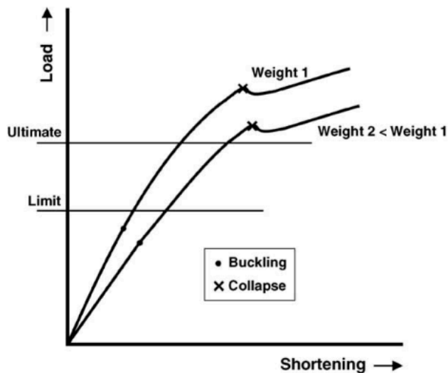
Fig. 2. Designs for first buckling under limit load and for postbuckling under ultimate load.
